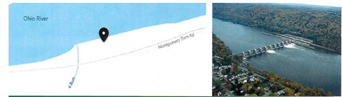
U.S. ARMY CORPS OF ENGINEERS - MONTGOMERY LOCKS & DAM SECANT PILE WALL CONSTRUCTION
